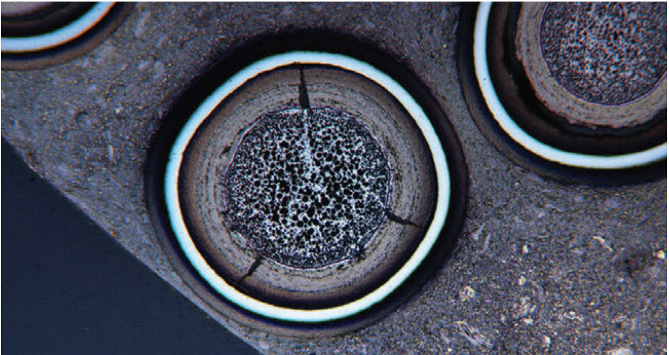
Individual TRISO fuel particles at 100um scale
